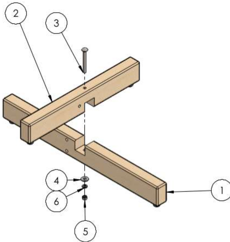
Figure 2a - Warping Wheel Base
