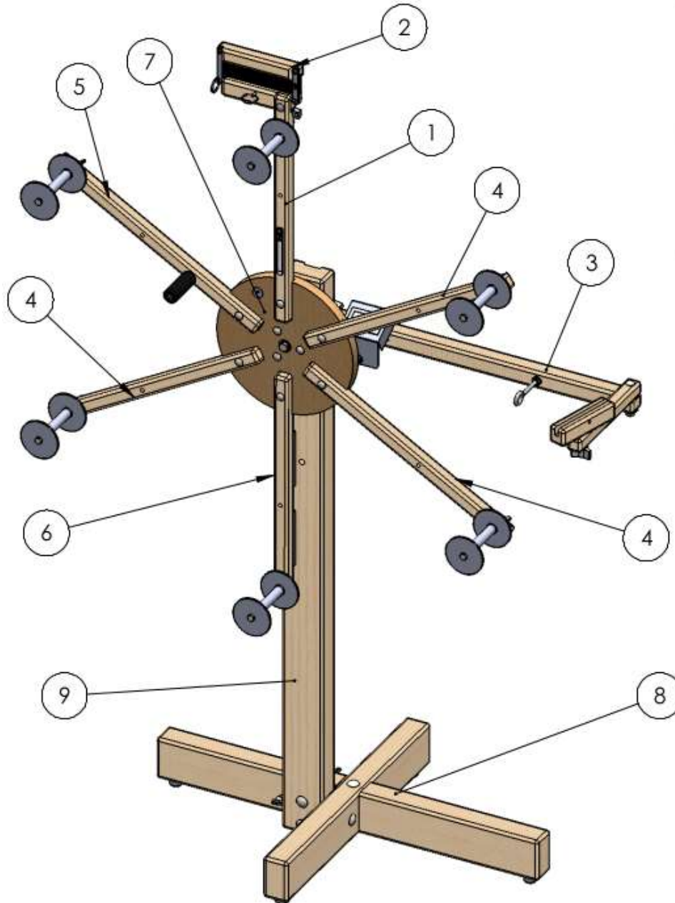
Figure 1 – Warping Wheel Parts
