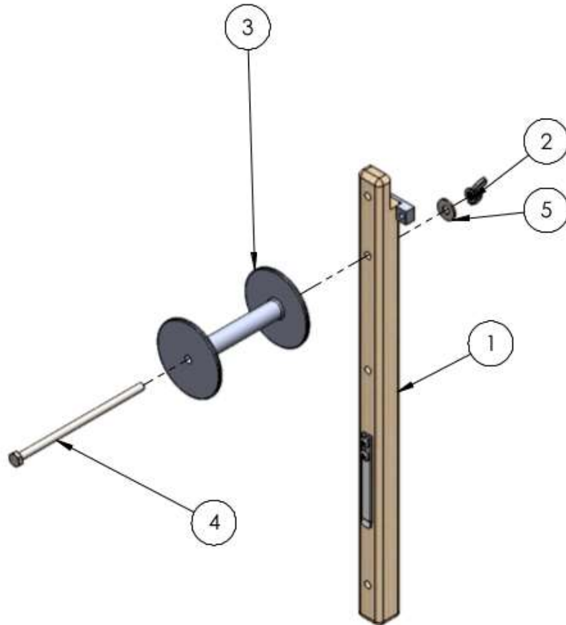
Figure 6 – Attach Spool to Spoke with clip
