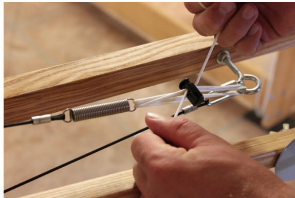
Figure 1 - Adjust Wind-off Tension
