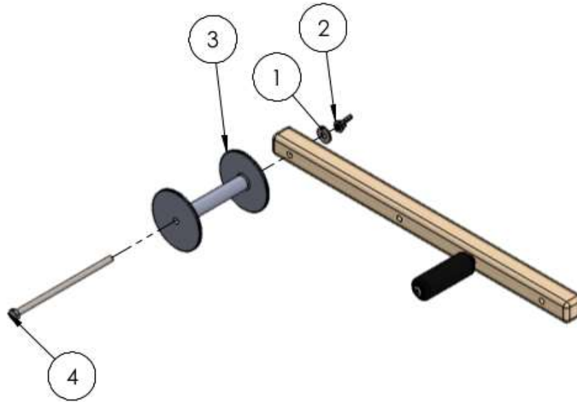
Figure 9a – Attach Spool to Spoke with handle
