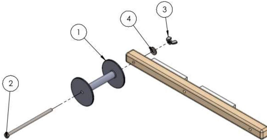
Figure 8a – Attach Spool to Weighted Spoke
