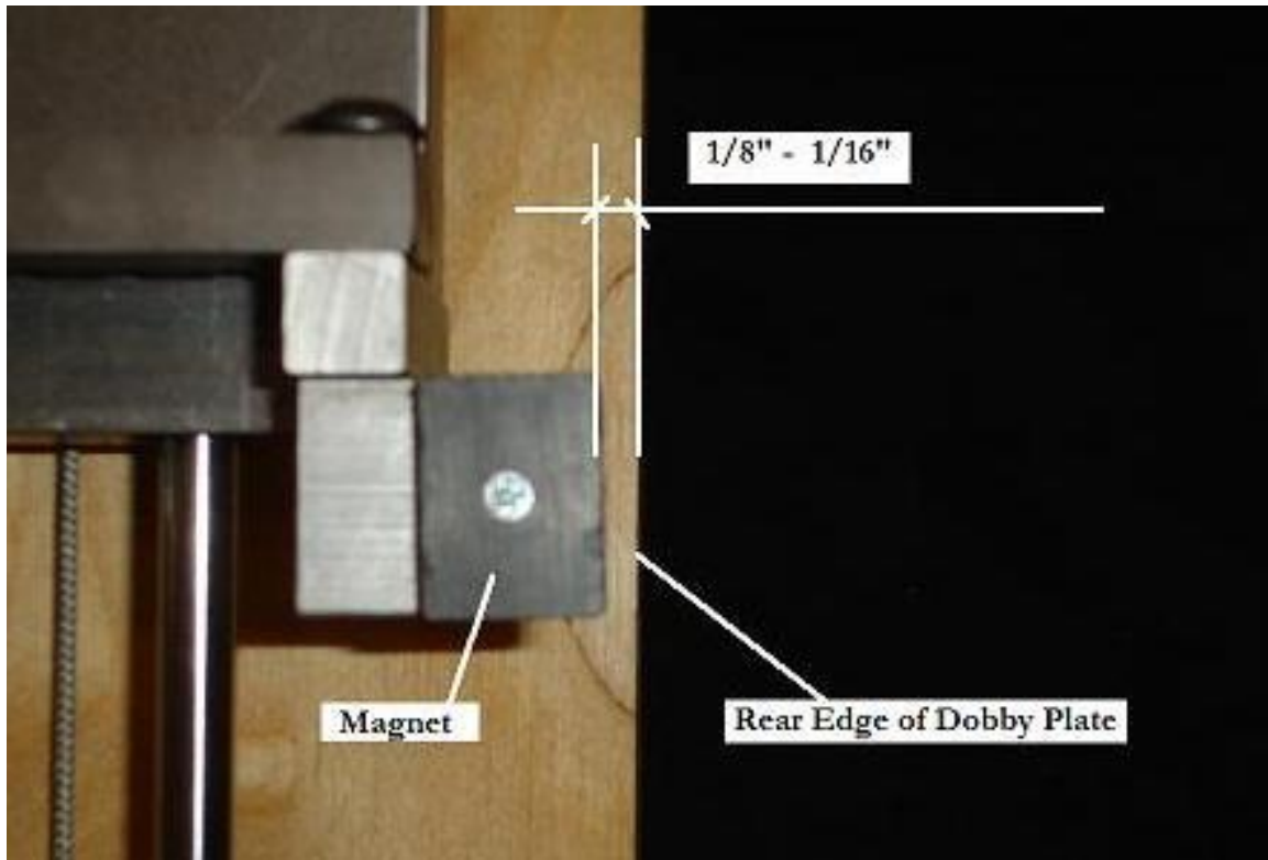
Fig. 1 – View looking straight on at the Magnet
