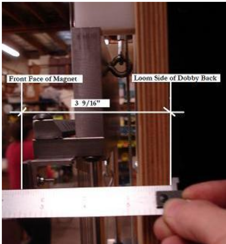
Fig. 2 – View from Side of Back Plate
